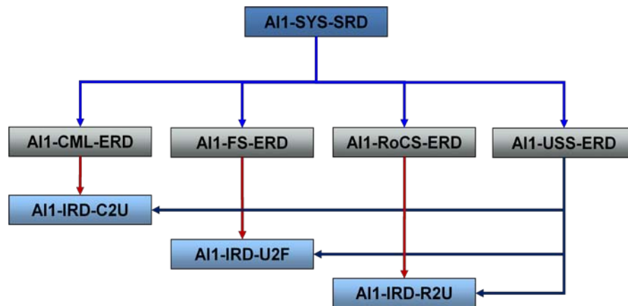
Figure 1 – System to Element to Interface Requirements Flow
