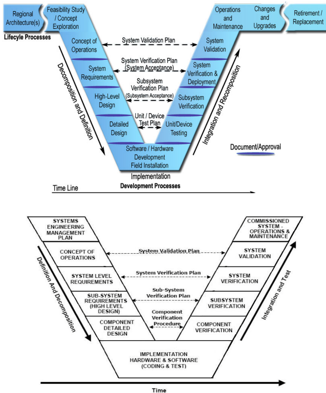
Figure 4 – Systems Engineering V-Diagram
