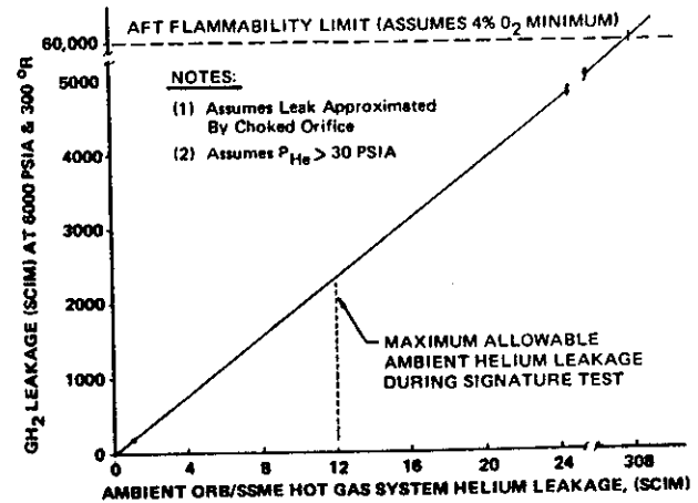
Figure 11. EQUIVALENT LEAKAGE RELATIONSHIP FOR HOT GAS SYSTEM, AMBIENT TO FLIGHT.
