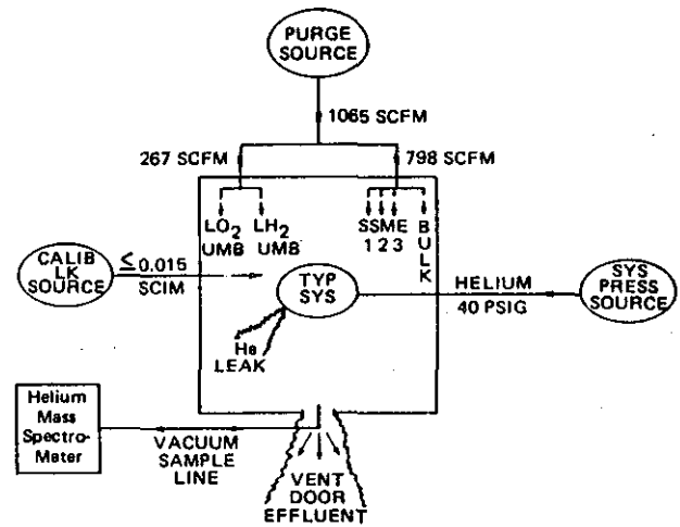
Figure 5. SCHEMATIC OF HELIUM SIGNATURE TEST SETUP
