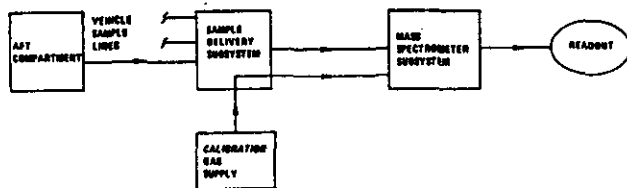
Figure 7. GROUND HAZARDOUS GAS DETECTION SYSTEM (HGDS) SCHEMATIC
